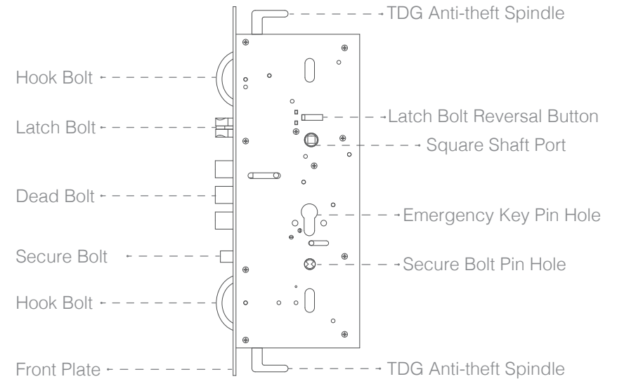
388 Lock Body (Optional)
