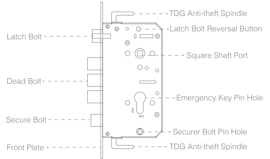
30 * 240 Lock Body (Optional)
